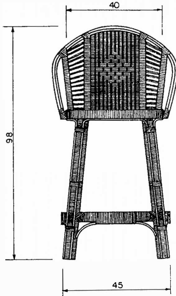
VISTA FRONTAL
