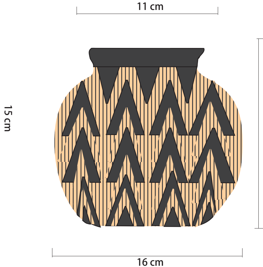
Vista Frontal
